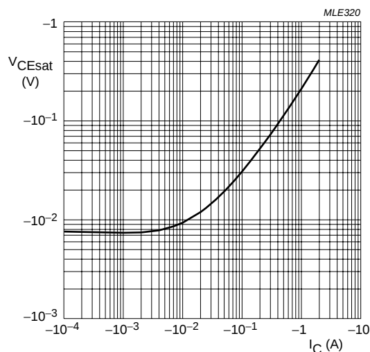
BC869-16.
