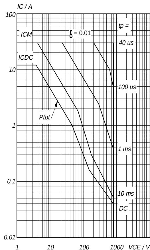
Fig.16. Forward bias safe operating area. T_{hs} = 25^\circ C I_{CDC} & I_{CM} = f(V_{CE}) ; I_{CM} single pulse; parameter t_p Second-breakdown limits independent of temperature. Mounted with heatsink compound.
