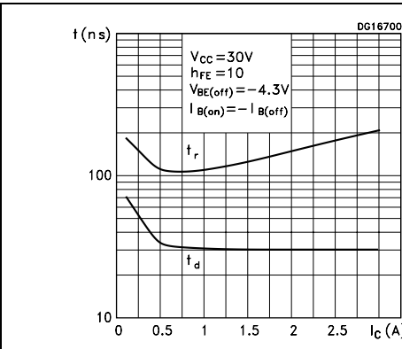
Figure 7. Resistive load switching time
