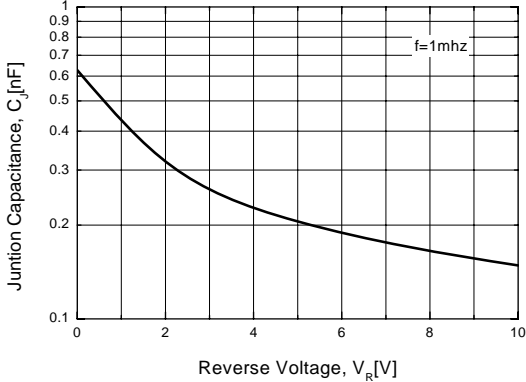
Figure 3. Junction Capacitance
