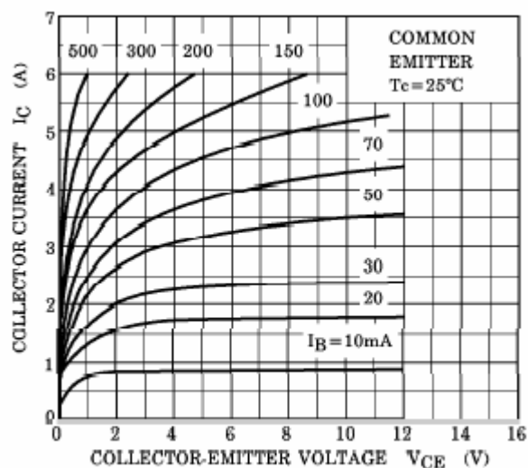
Fig.3 Static Characteristic
