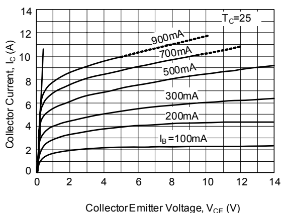
Collector Output Characteristics
