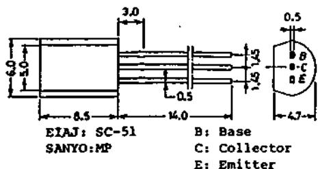
Case Outline—[2008A]
