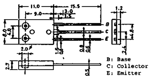
Case Outline—[2043A] unit:mm
