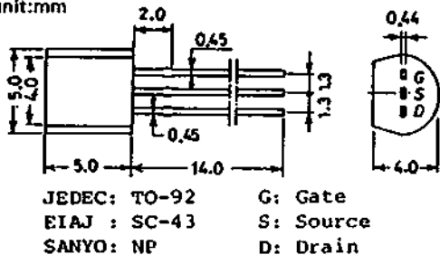
Case Outline—[2008A]
