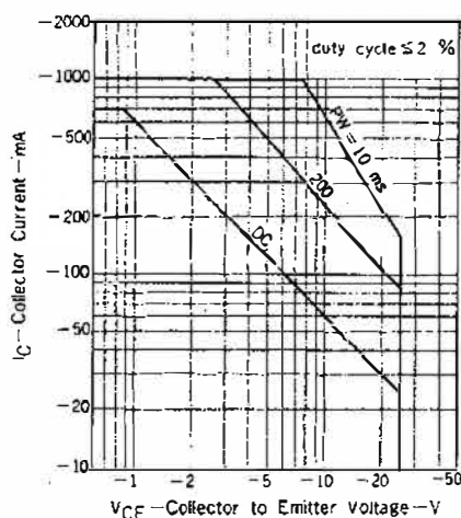
SAFE OPERATING AREAS (TRANSIENT THERMAL RESISTANCE)
