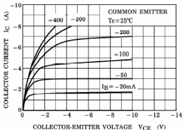
Fig.3 Static Characteristic
